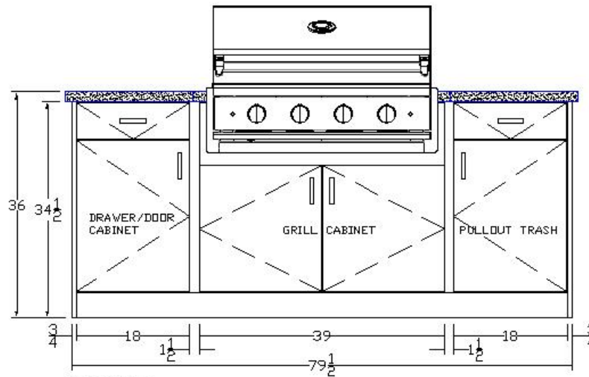
ELEVATION STRAIGHT RUN - 2 PREP AREA
