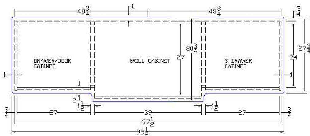
PLAN VIEW STRAIGHT RUN - 2 PREP AREA WITH DRAWERS (ISLAND)
