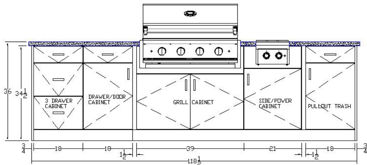
ELEVATION STRAIGHT RUN - 2 PREP AREAS & BURNER
