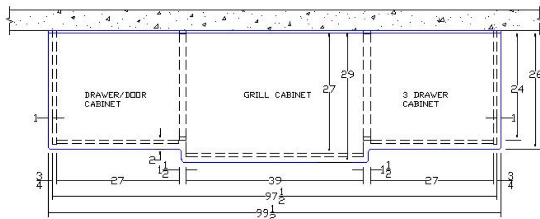
PLAN VIEW STRAIGHT RUN - 2 PREP AREA WITH DRAWERS (AGAINST WALL)
