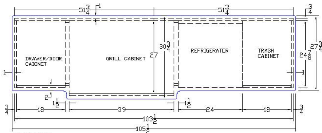
PLAN VIEW STRAIGHT RUN - 2 PREP AREAS & 24" REFRIGERATOR (ISLAND)
