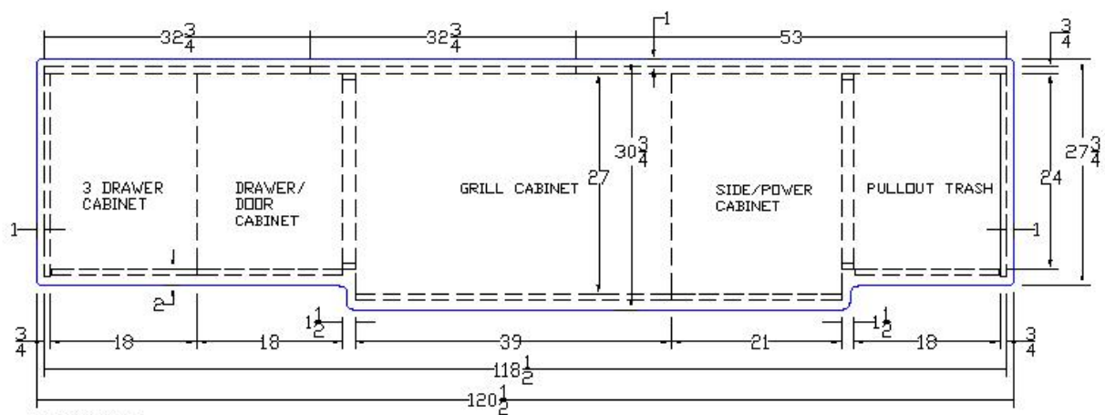
PLAN VIEW STRAIGHT RUN - 2 PREP AREAS & BURNER (ISLAND)
