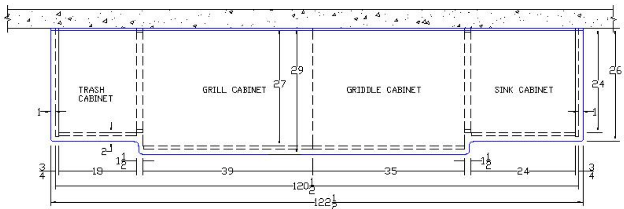
PLAN VIEW STRAIGHT RUN - 2 PREP AREAS & 1 GRILL/1 GRIDDLE (AGAINST WALL)
