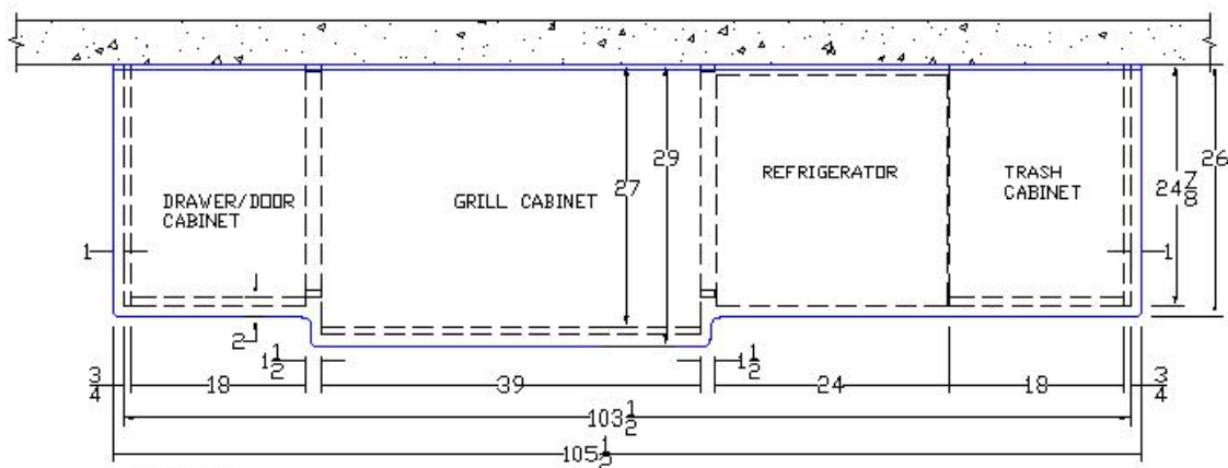
PLAN VIEW STRAIGHT RUN - 2 PREP AREAS & 24" REFRIGERATOR (AGAINST WALL)
