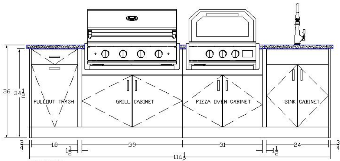
ELEVATION STRAIGHT RUN - 2 PREP AREAS & 1 GRILL/1 PIZZA OVEN
