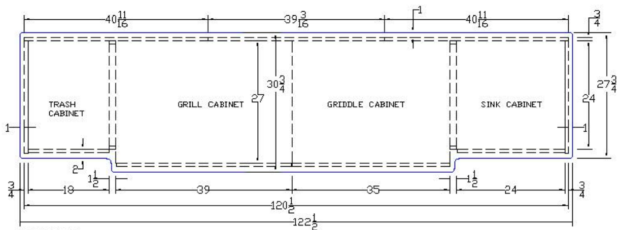
PLAN VIEW STRAIGHT RUN - 2 PREP AREAS & 1 GRILL/1 GRIDDLE (ISLAND)
