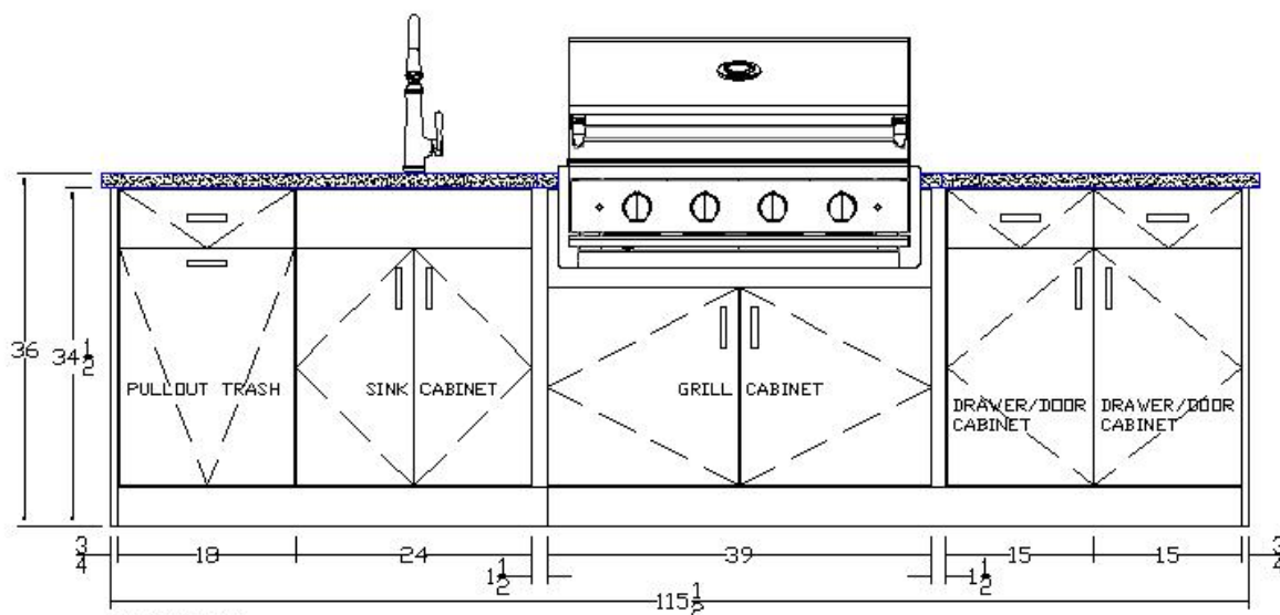
ELEVATION STRAIGHT RUN - 2 PREP AREAS & SINK
