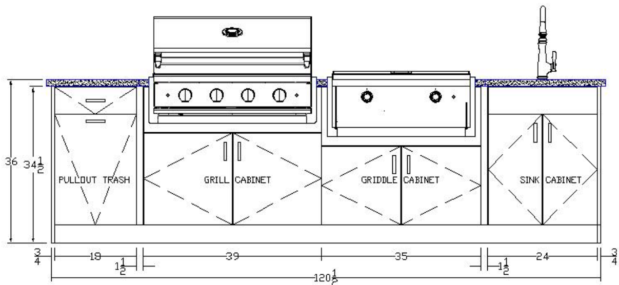
ELEVATION STRAIGHT RUN - 2 PREP AREAS & 1 GRILL/1 GRIDDLE
