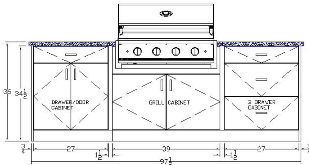
ELEVATION STRAIGHT RUN - 2 PREP AREA WITH DRAWERS
