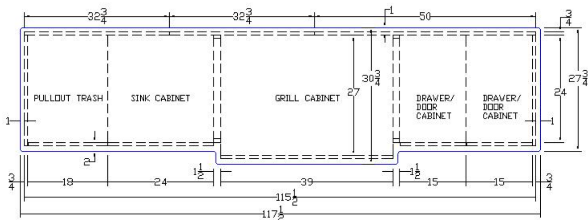
PLAN VIEW STRAIGHT RUN - 2 PREP AREAS & SINK (ISLAND)
