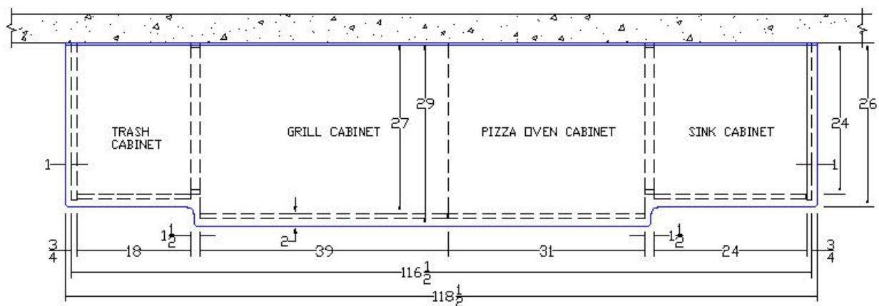
PLAN VIEW STRAIGHT RUN - 2 PREP AREAS & 1 GRILL/1 PIZZA OVEN (AGAINST WALL)
