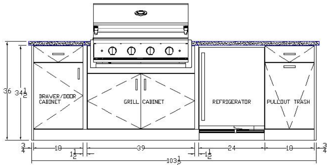
ELEVATION STRAIGHT RUN - 2 PREP AREAS & 24" REFRIGERATOR
