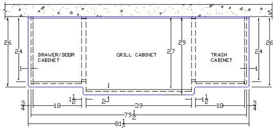
PLAN VIEW STRAIGHT RUN - 2 PREP AREA (AGAINST WALL)
